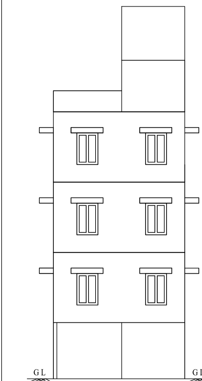
FRONT ELEVATION
